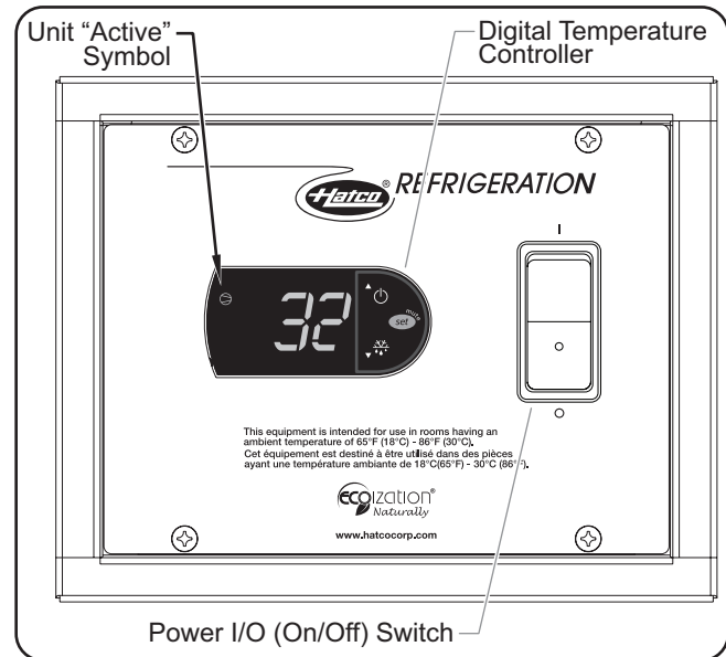
CWB Series Control Box
