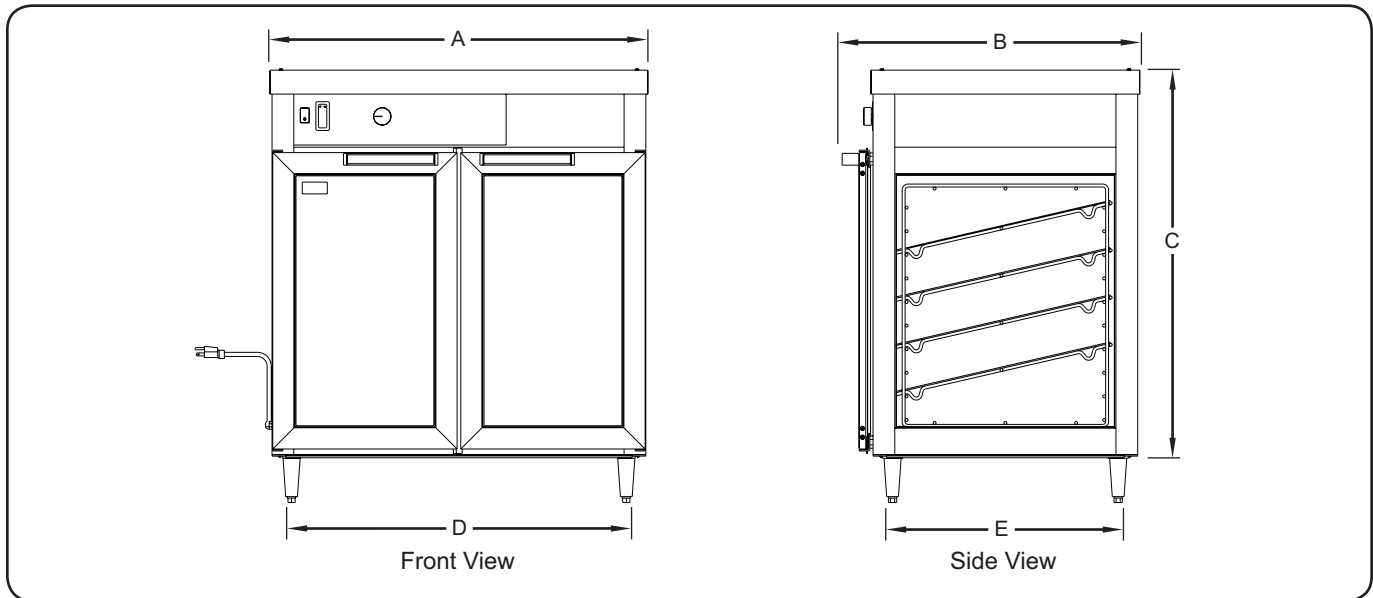
WFST-1X Dimensions
