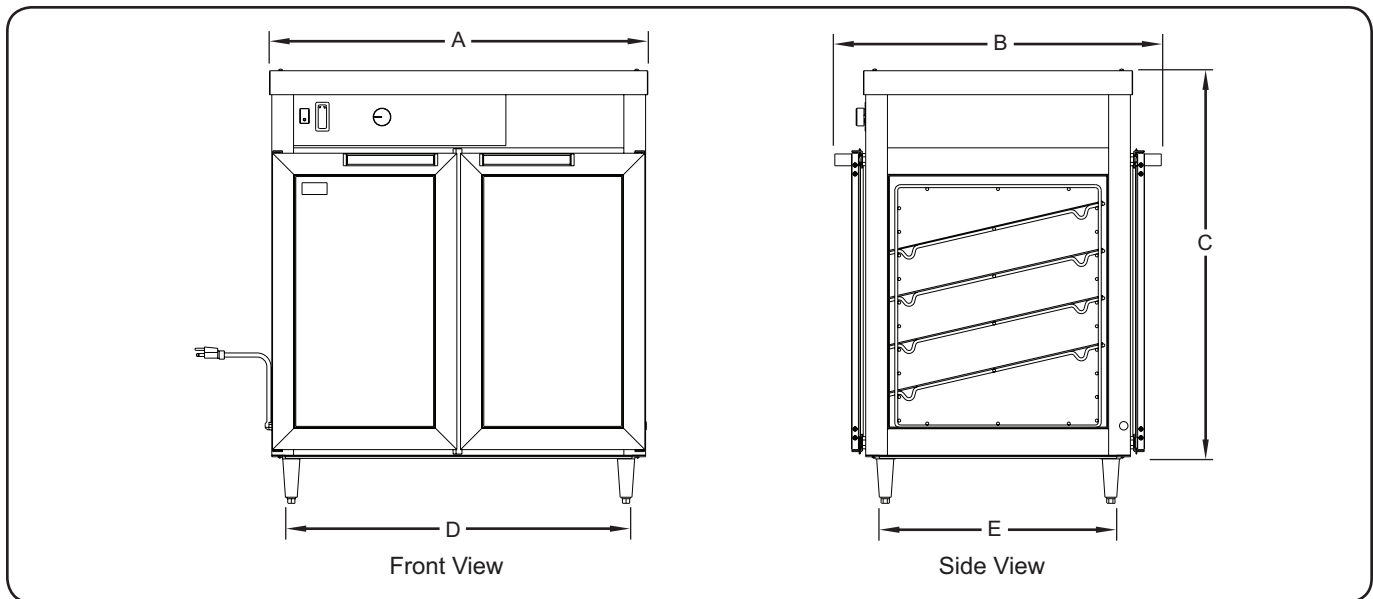
WFST-2X Dimensions
