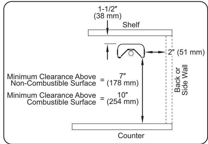
Minimum Clearances
