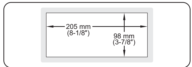
Control Box Cutout Dimensions
