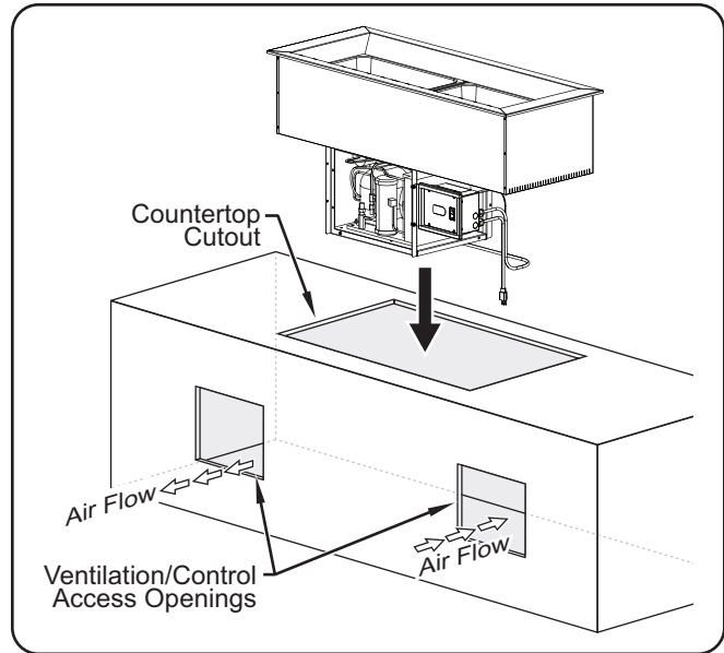
Installing a CWB-S2 Model
