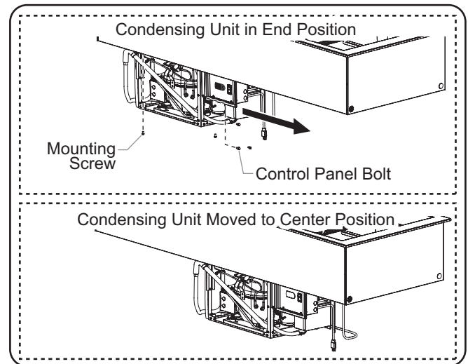
Moving a CWB-S4 Model Condensing Unit
