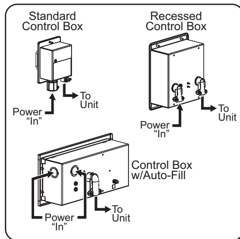
Control Enclosure Electrical Connections
