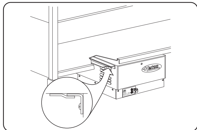
Compact Series Heater Mounted to Dishtable
