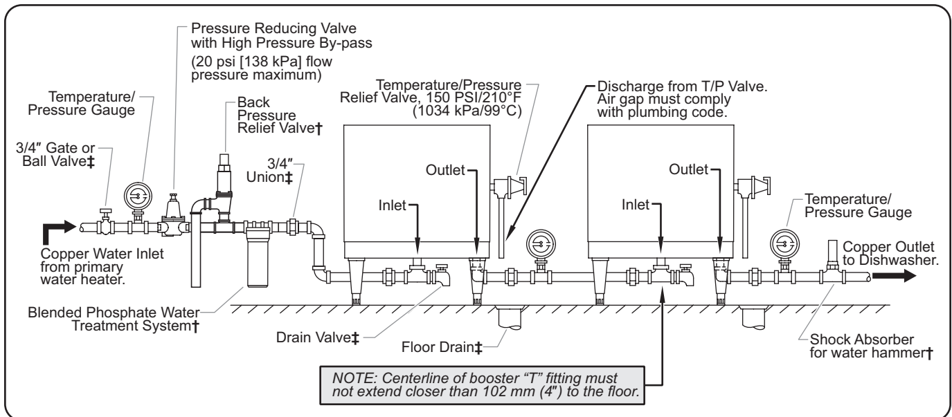
Two Imperial Models Connected in Series
