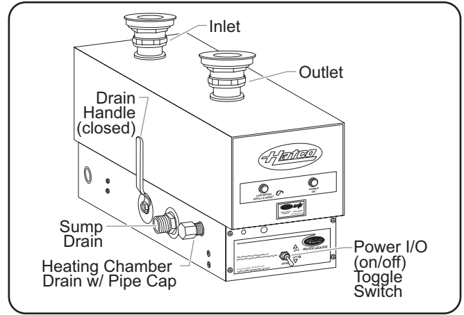
3CS Model
