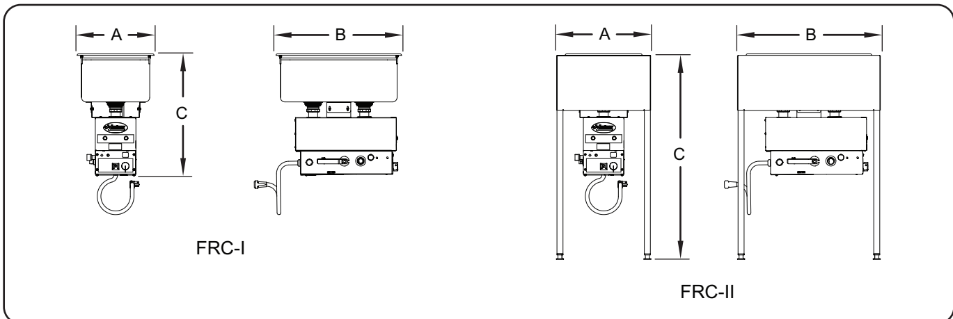
Dimensions—FRC Models
