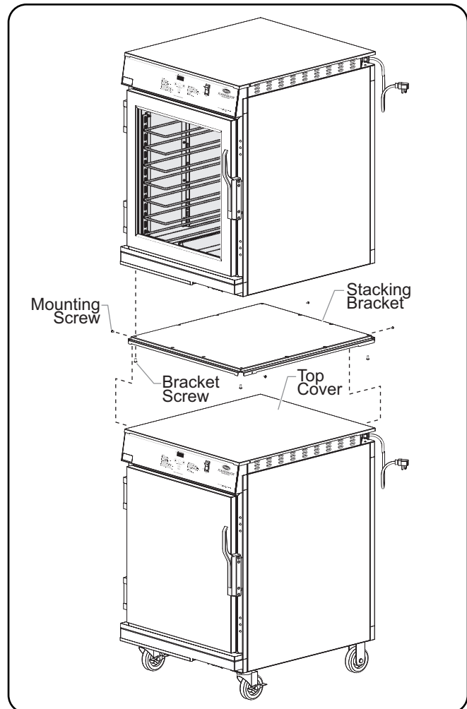
Stacking two units (FSHC-TW1-EE shown)
