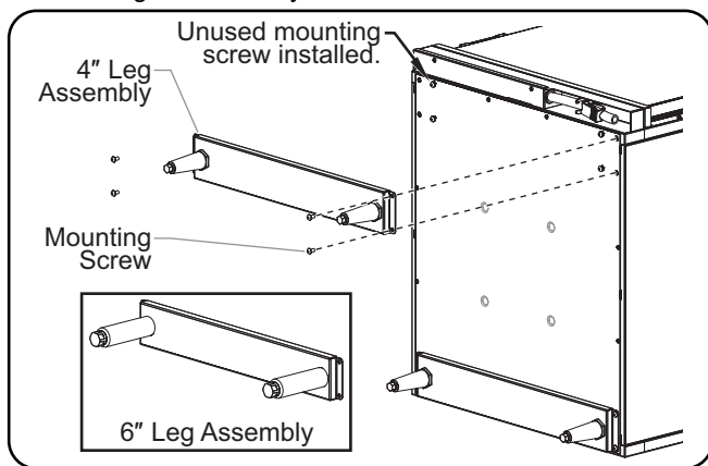
Installing Legs
