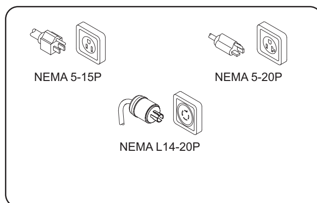
Plug Configurations
