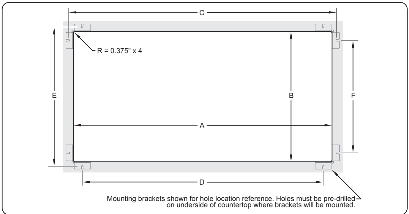
Countertop Cutout and Mounting Bolt Dimensions
