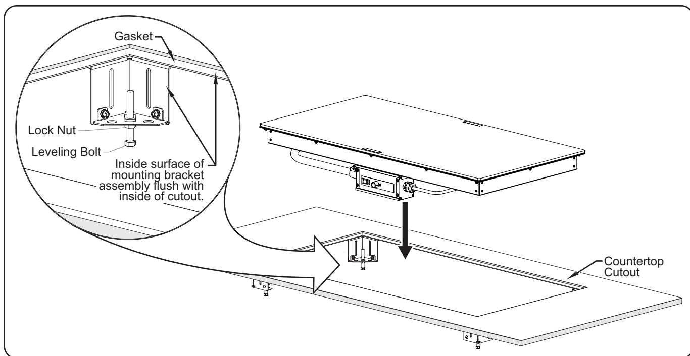
Installing an HSBF Series Heated Shelf
